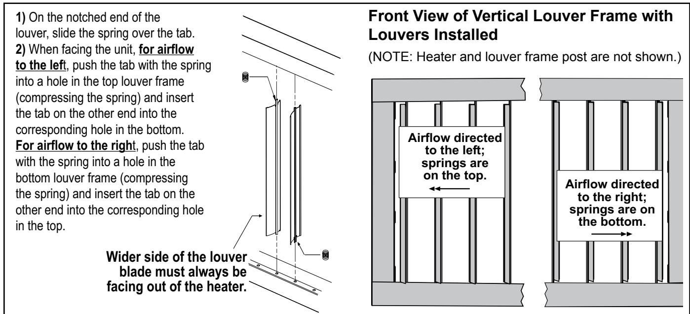
FIGURE 2 - Installing Louvers
